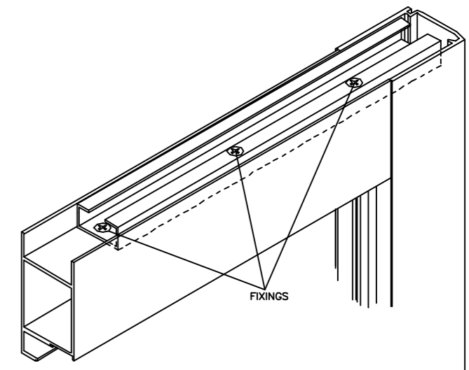
HANGER CHANNEL FIXING
