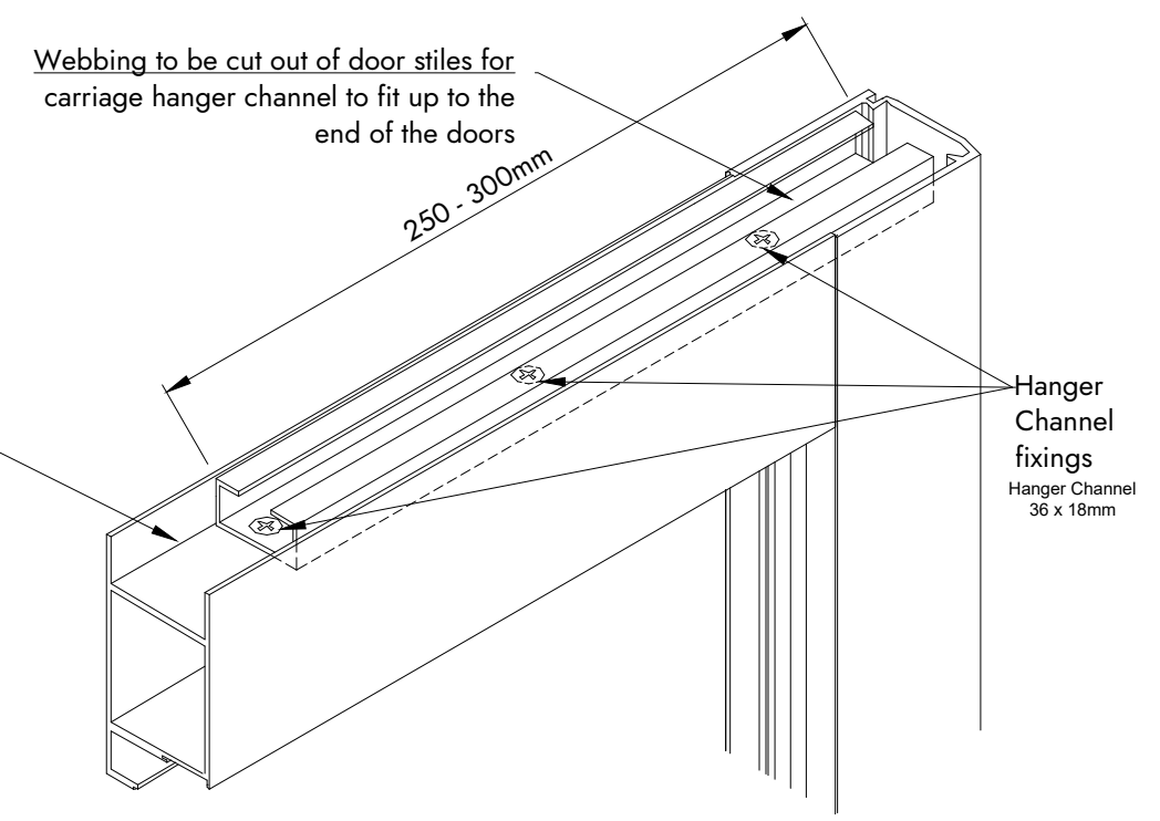
CARRIAGE HANGER CHANNEL FIXING
