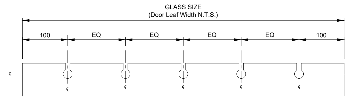
FRAMELESS GLASS HOLE SETOUT FOR GLASS DOOR WEIGHT UP TO 400kg
